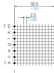
Grid View pin-side
